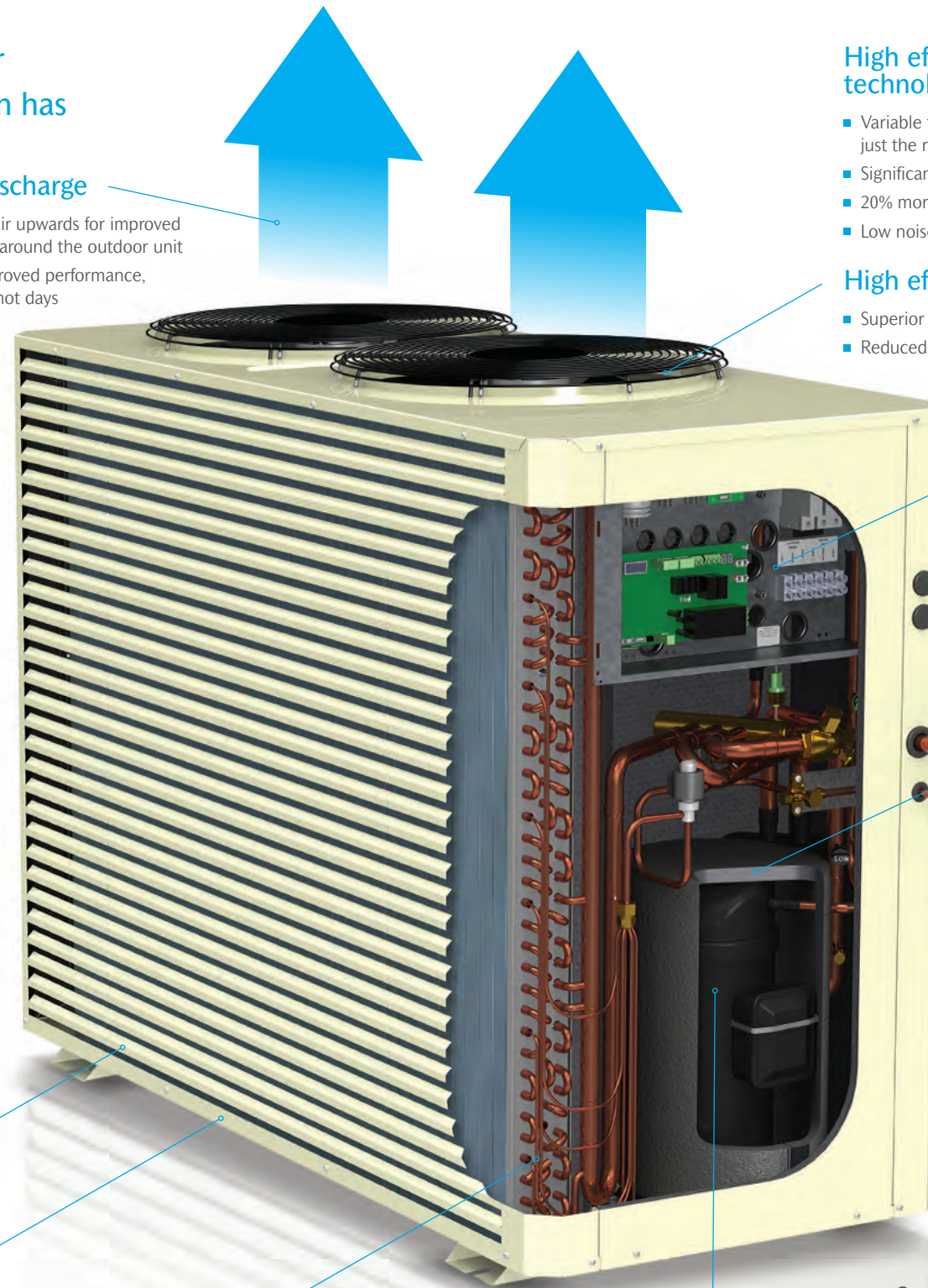
Outdoor Unit
